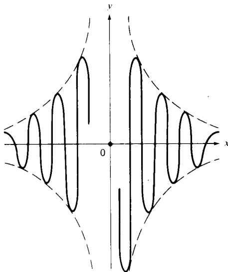
Figure 2.5 y = (1/x) \cos(1/x) .
