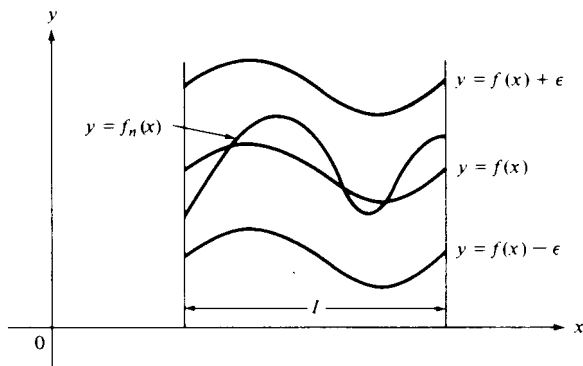
Figure 8.1 Illustrating uniform convergence.
