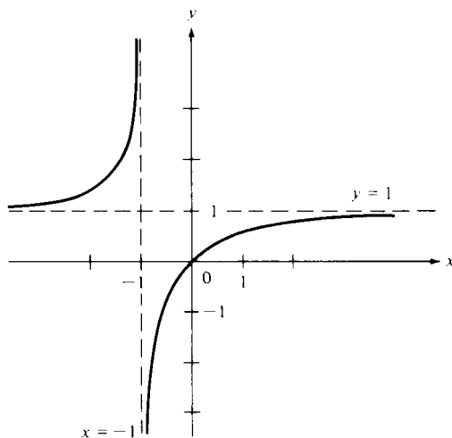
Figure 2.4 y = x/(x + 1) .
